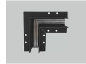
L shape connector (90° Corner) 1292-RT-CON-L Dimensions 109*109*55 Cut-out 109*109*35 DC24V
