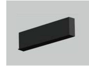
Adaptor Kit for surface mounted track 1292-STAK-80 Dimensions 441*55*27 DC24V
